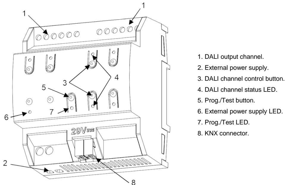
Figure 2. Element Diagram.
