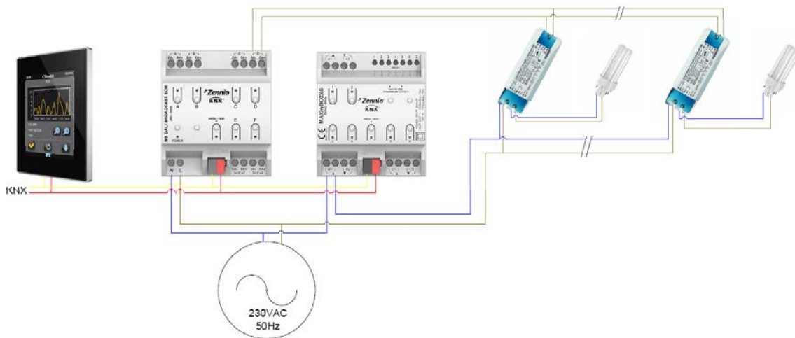
Figure 20. Standby Scheme
