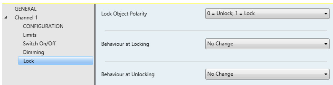
Figure 18. Channel “x”. Lock
