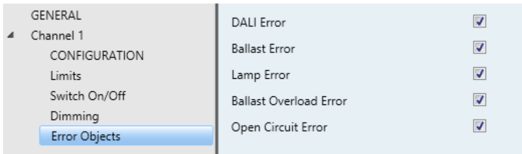
Figure 8. Channel “x”. Error Objects
