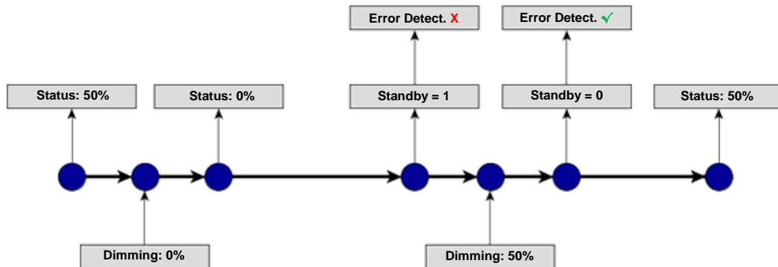
Figure 21. Standby mode action sequence
